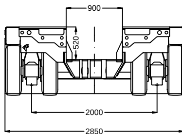
Frontansicht / front view
